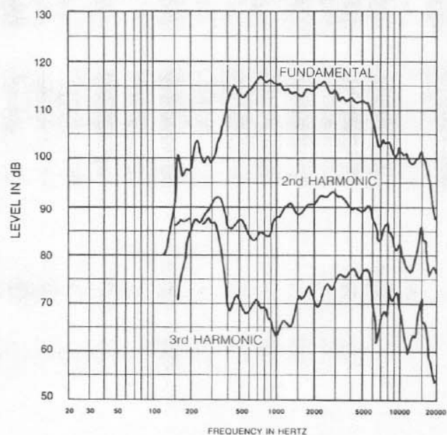
FIGURE 5 Distortion Response, HP9040 Horn, 3 Watts/1 Meter
