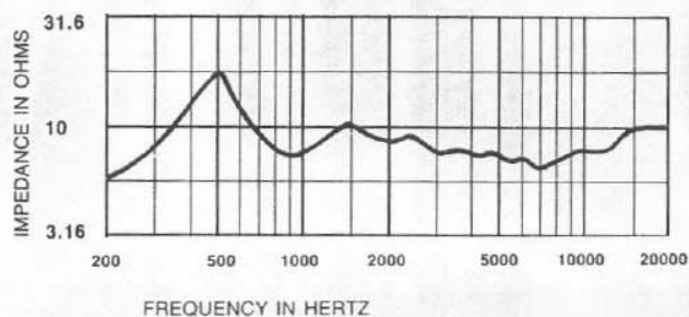
FIGURE 6 Impedance Response — 1-Inch Plane-Wave Tube
