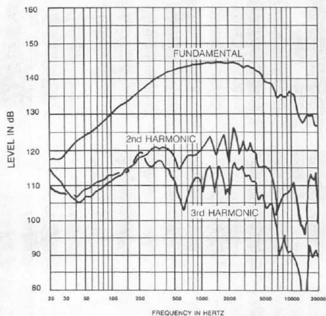
FIGURE 4 Distortion Response, 1-Inch Plane-Wave Tube, 3 Watts
