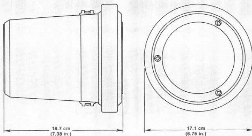
FIGURE 2 Dimensions
